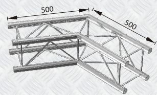
GT F2J22 120° CORNER
