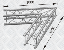
GT F24J20 60° CORNER
