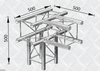
GT F24J40 4 WAY 'T' TO VERTICAL JUNCTION
