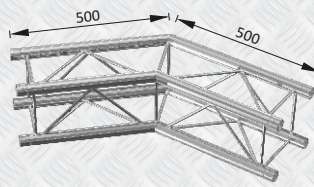
GT F24J23 135° CORNER
