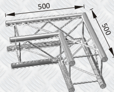
GT F24J21 90° CORNER
