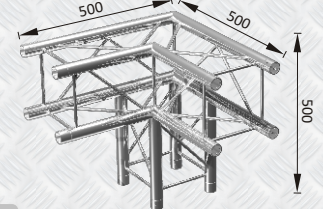
GT F24J30 3 WAY 90° CORNER TO VERTICAL JUNCTION
