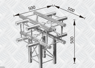
GT F24J55 5 WAY 'X' TO VERTICAL JUNCTION
