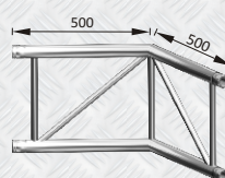
GT F42PJ22-V 120° VERTICAL CORNER
