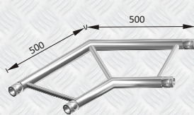
GT F42PJ22-H 120° HORIZONTAL CORNER
