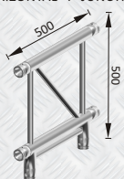
GT F42PJ36-H HORIZONTAL 'T' JUNCTION
