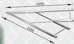
GT F42PJ19-H 45° HORIZONTAL CORNER
