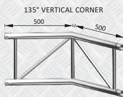
GT F42PJ23-V 135° VERTICAL CORNER
