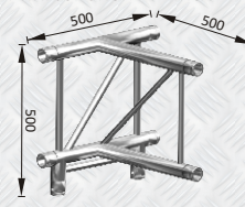
GT F42PJ42-V 4 WAY JUNCTION - VERTICAL
