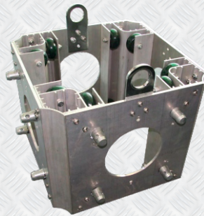
F34 SLEEVE BLOCK (CAN CARRY F33, F34 & F44 BEAMS)
