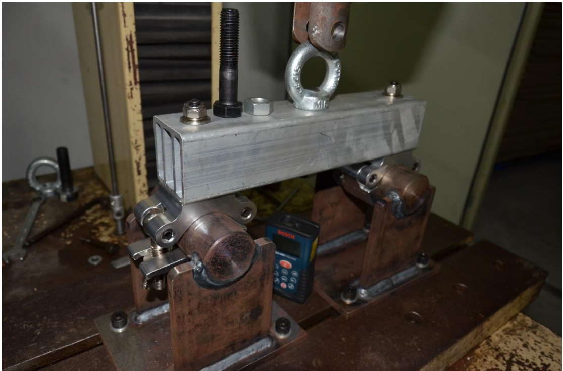
Distance is 0.163m after loaded deformation of the specimen at five minutes
