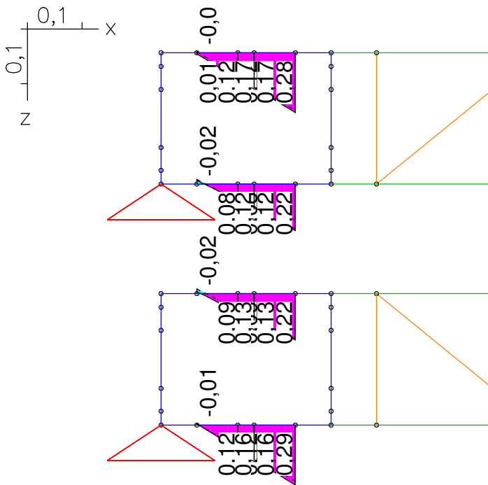
Internal forces My min, max; LFK K100, ULS
