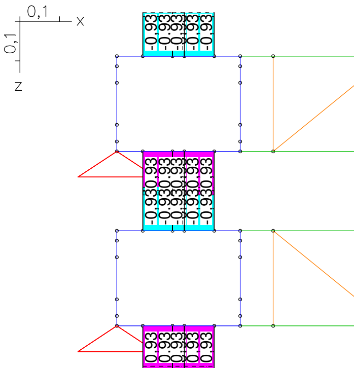
Internal forces Nx min, max; LFK K100, ULS
